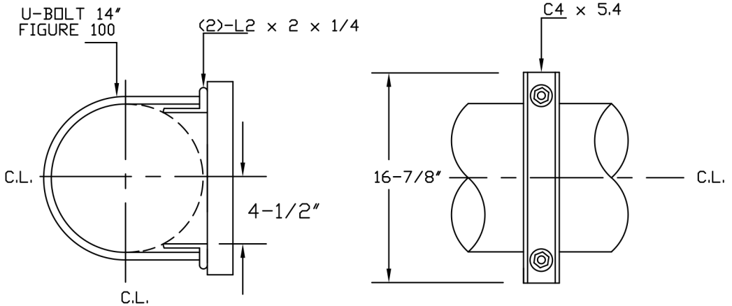
14" LINE
