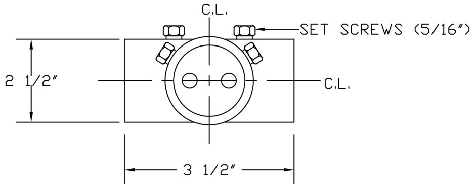
END VIEW
